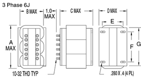
Diagram 1, (Suffix A)
