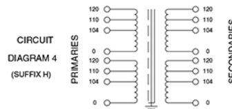
Diagram 4, (Suffix H)
