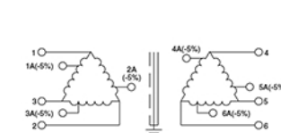
Diagram 4, (Suffix H)
