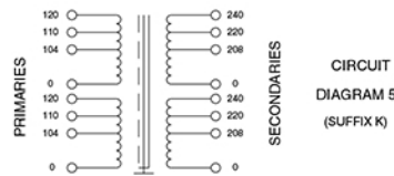
Diagram 5, (Suffix K)
